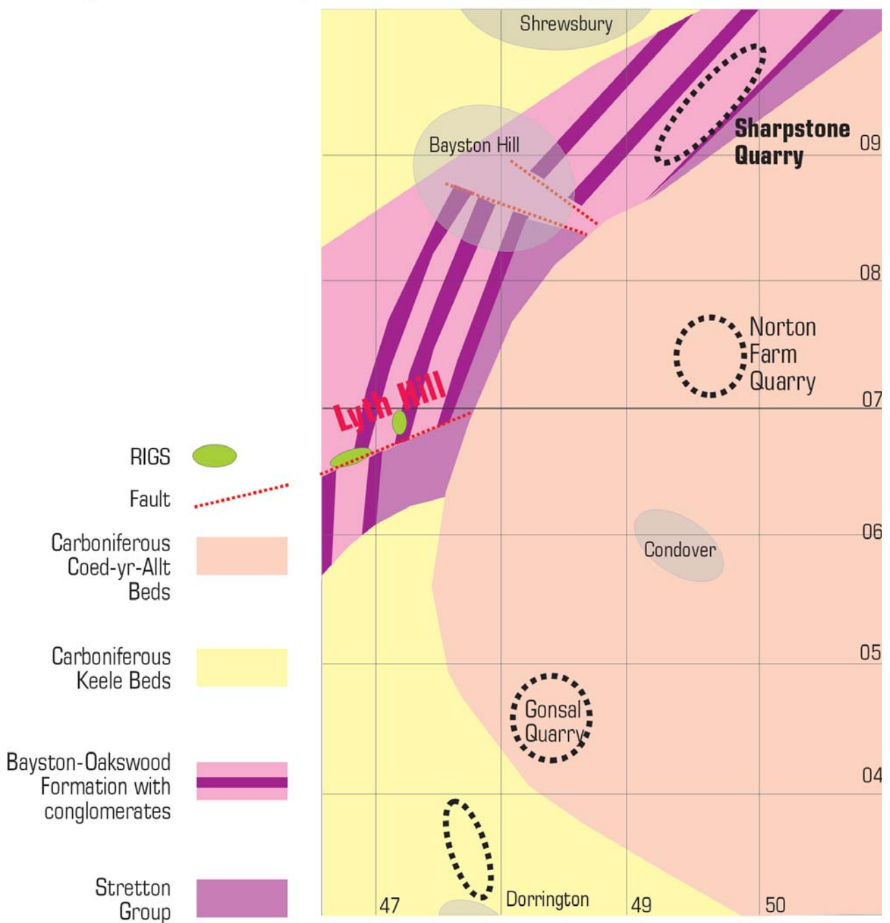
Diagrammatic map of the solid geology around Lyth Hill
